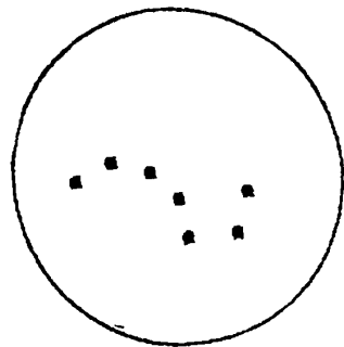
Fig. 17. Adjusted Guess
